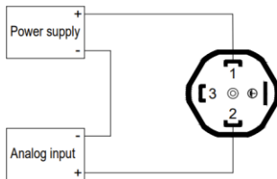
2-wire / current
