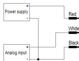
3-wire / voltage
