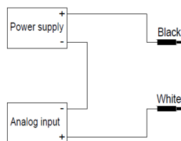
2-wire / current
