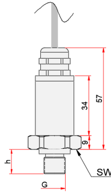
Cable gland type
