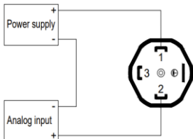
2-wire / current
