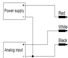
3-wire / voltage
