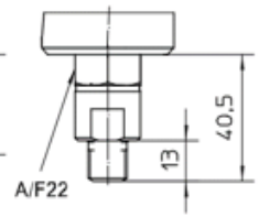
BSPT 1/4"
