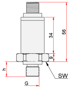
M12 Plug type
