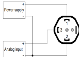
3-wire / voltage
