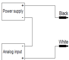
2-wire / current
