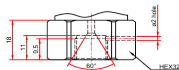
9/16-18 UNF Seal cone BOSS SAE J514
