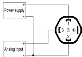
3-wire / voltage
