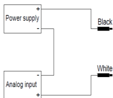
2-wire / current
