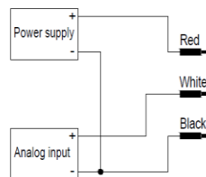
3-wire / voltage
