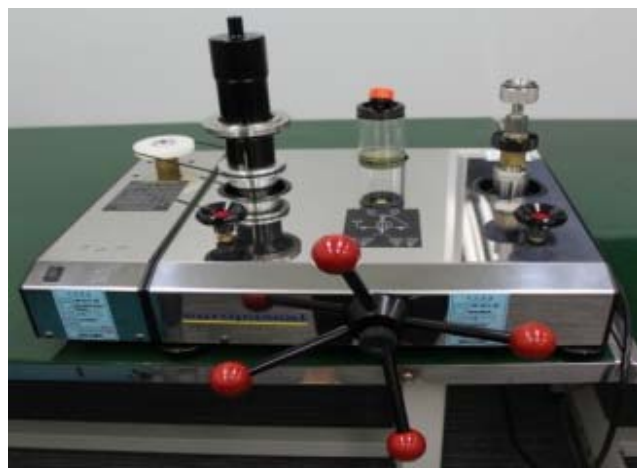
Europascal Hydraulic DWT-BH2-D-1200 Max.1200bar / 0.007% of rdg.
