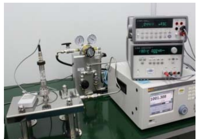
Fluke Controller PPC4EX-100K ±15kPa & 200kPa abs / 0.005% of F.S
