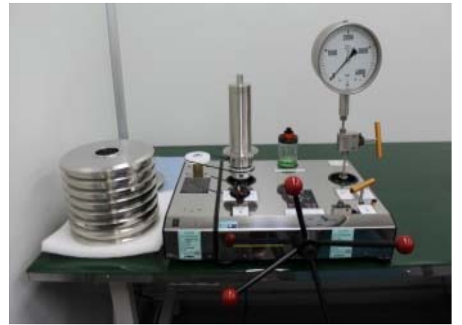
Europascal Hydraulic DWT-BH2-4000 Max.4,000bar / 0.015% of rdg.
