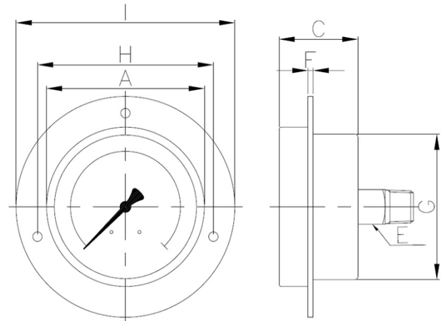
BD : Back connection with Front Flange
